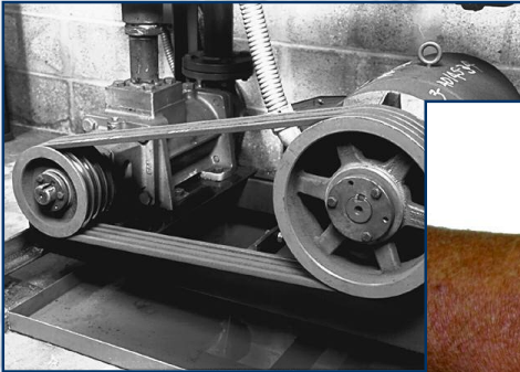
DANGEROUS SAFETY VIOLATION - NO GUARD OVER THE BELTS.
